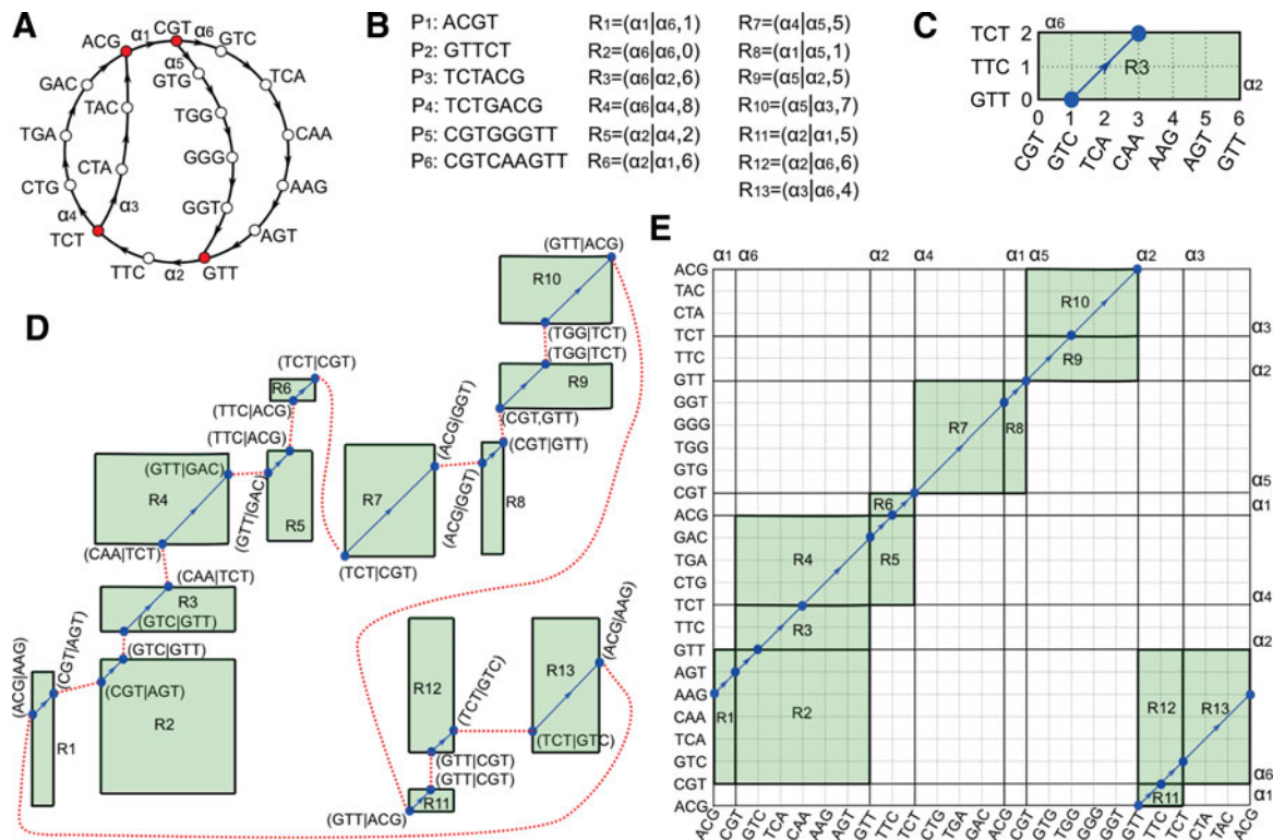
FIG. 4. Construction of the paired assembly graph for bireads sampled from a circular 24 bp genome \text{GENOME} = \text{ACGTCAAGTTCTGACGTGGGTTCT} (single reads referred to as \text{READS} ). The de Bruijn graph \text{DB}(\text{READS}, 4) has four hubs (ACG, CGT, GTT, and TCT) (A) and six h-paths P_1, \dots, P_6 , with lengths 1, ..., 6 respectively (B). The h-edge of path P_i , denoted \alpha_i , is its first edge. The cycle C in \text{DB}(\text{READS}, 4) that spells \text{GENOME} passes through the h-paths in order P_1, P_6, P_2, P_4, P_1, P_5, P_2, P_3 ( P_1 and P_2 represent repeats). (B) Reads are paired with separation d = 5 , yielding estimated distances D between various h-edges \alpha_i and \alpha_j , denoted as the h-biedge (\alpha_i|\alpha_j, D) . The 13 h-biedges constructed from all bireads are listed as R_1, \dots, R_{13} . (C) The rectangle diagram of h-biedge (\alpha_6|\alpha_2, 6) is a rectangle ( R_3 ) with sides P_6 and P_2 and 45^\circ line segment y = x + (d - 4) = x - 1 , from (1, 0) to (3, 2). Point (1, 0) is labeled by bivertex (GTC|GTT) formed by vertex 1 (GTC) in path P_6 and vertex 0 (GTT) in path P_2 . Point (3, 2) is labeled by bivertex (CAA|TCT) formed by vertex 3 (CAA) in path P_3 and vertex 2 (TCT) in path P_2 . (D) Vertices from different rectangle diagrams are indicated by dotted red lines. (E) Rectangles glued into a 24 \times 24 grid, yielding a cycle (blue path) through the genome.
